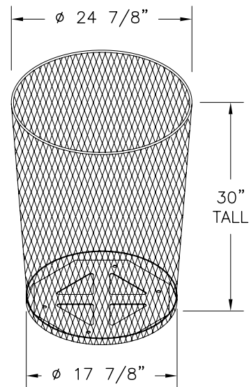
TAPERED RECEPTACLE DIMS
