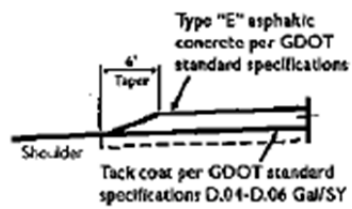
Shoulder detail for streets without curbs
