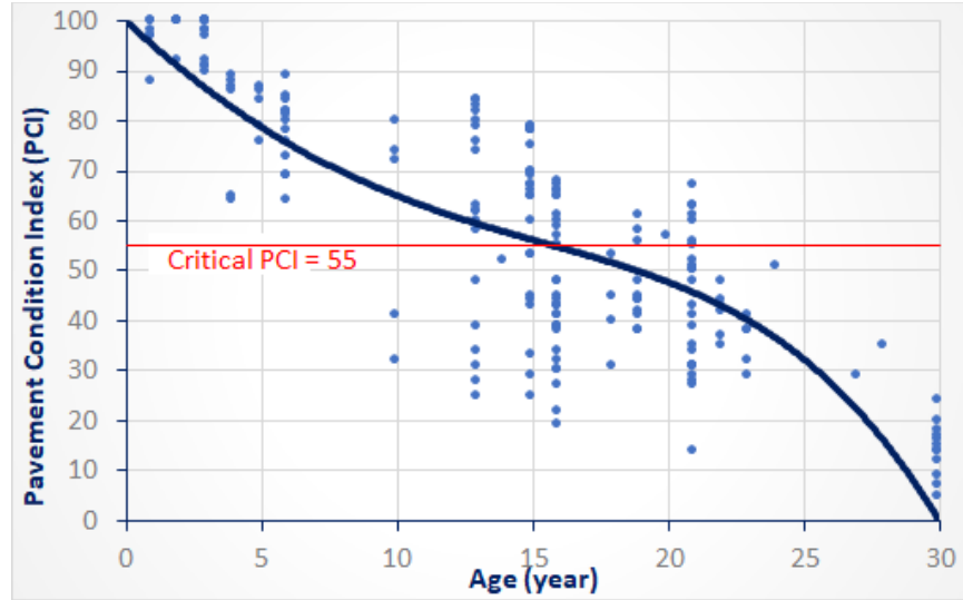
A Sample Pavement Performance Model
