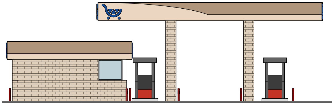
3 A12 LEFT ELEVATION 3/32" = 1'-0"
