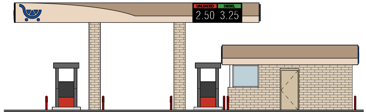
4 A12 RIGHT ELEVATION 3/32" = 1'-0"
