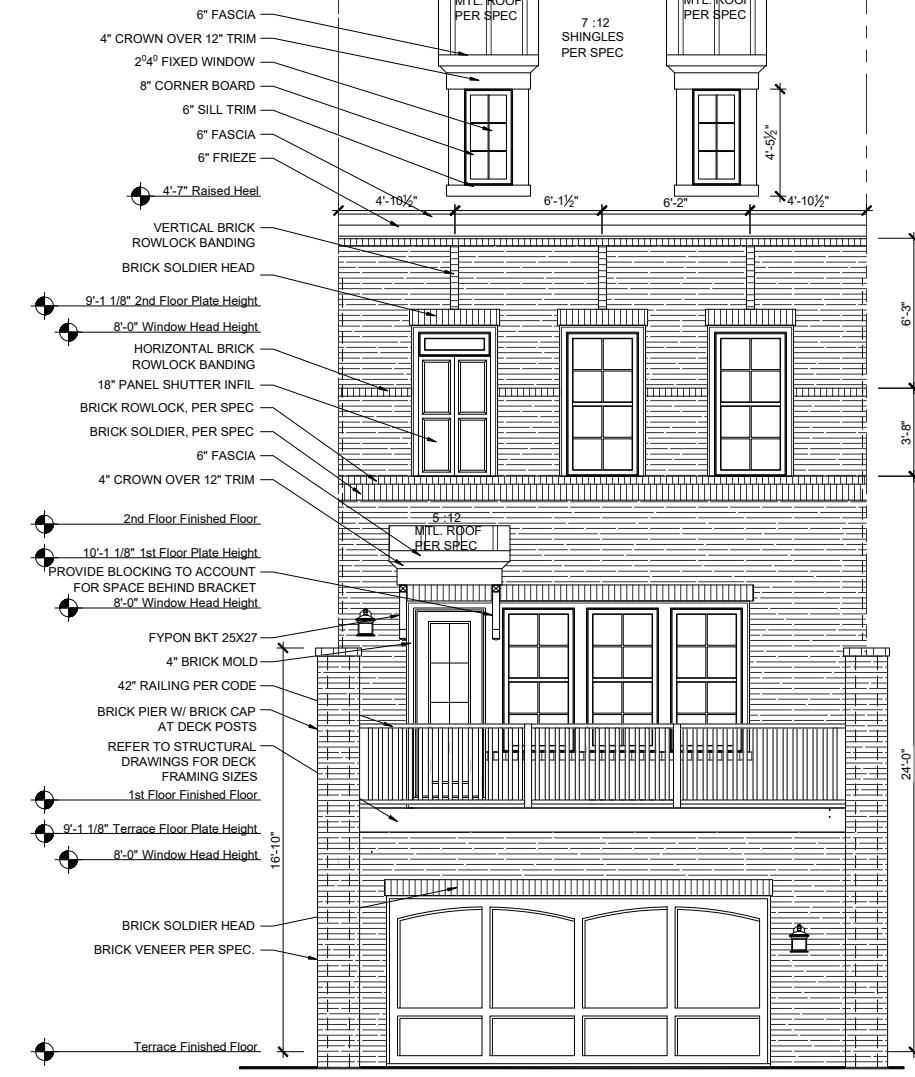
REAR ELEVATION - F - GRADE ENTRY DUAL OWNER SCALE: 1/8"=1'-0" (11"x17" SHEET SIZE) SCALE: 1/4"=1'-0" (22"x34" SHEET SIZE)
