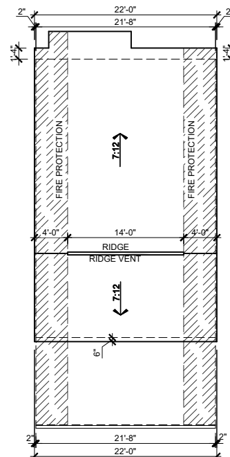
ROOF PLAN - C SCALE: 1/16"=1'-0" (11"x17" SHEET SIZE) SCALE: 1/8"=1'-0" (22"x34" SHEET SIZE)
