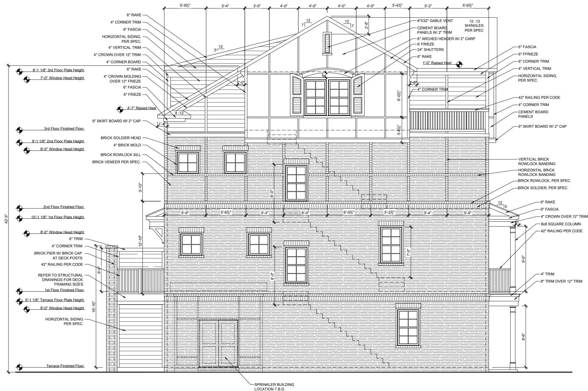
SIDE ELEVATION GRADE ENTRY SCALE: 1/8"=1'-0" (11"x17" SHEET SIZE) SCALE: 1/4"=1'-0" (22"x34" SHEET SIZE)
