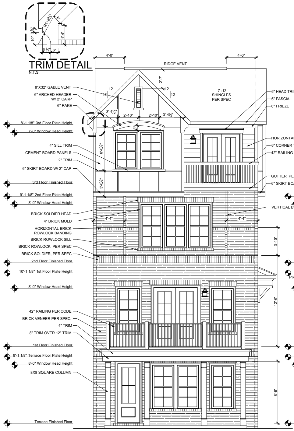
FRONT ELEVATION - F - 1st GRADE ENTRY SCALE: 1/8"=1'-0" (11"x17" SHEET SIZE) SCALE: 1/4"=1'-0" (22"x34" SHEET SIZE)
